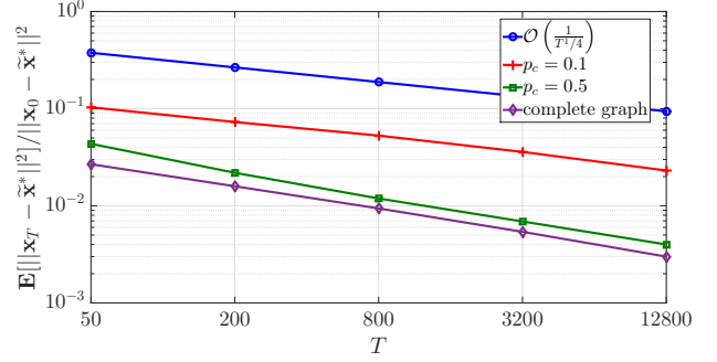
Fig. 2. Relative optimal squared error for three vales of graph connectivity ratio: p_c \in \{0.1, 0.5, 1\} , compared with the order of upper bound.
